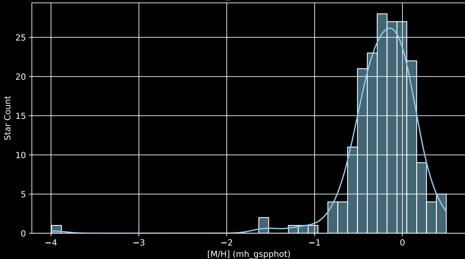
APOGEE DR17 Field: [077+45_MGA [M/H] (mh_gspphot) (n= 191)
