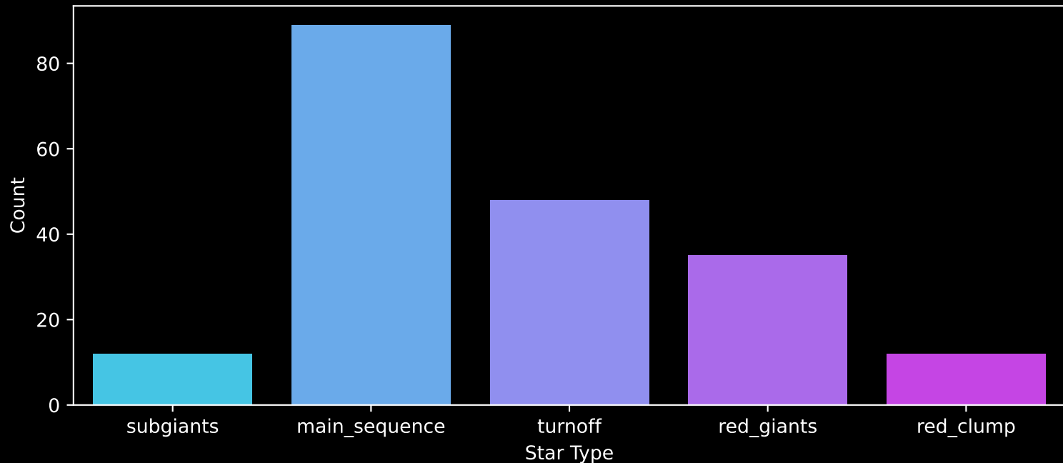
Count plot of Star Type
