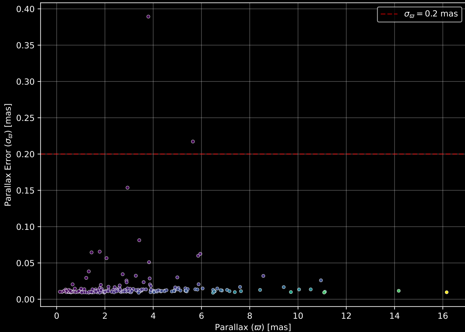
APOGEE DR17 Field: [077+45_MGA] Parallax Quality (n= 196)
