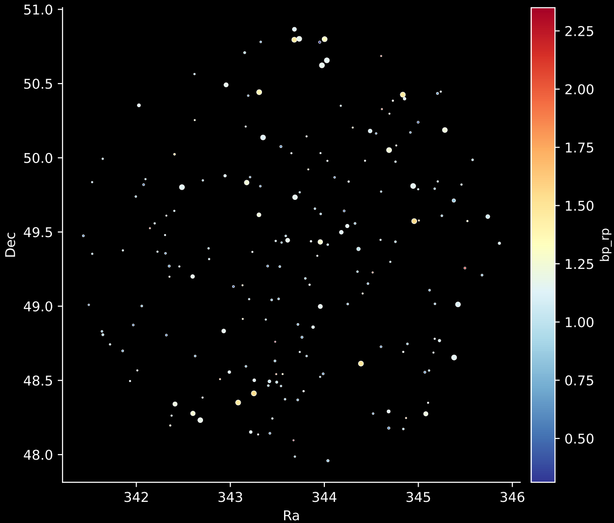
APOGEE DR17 Field: [077+45_MGA] Stars: 196
