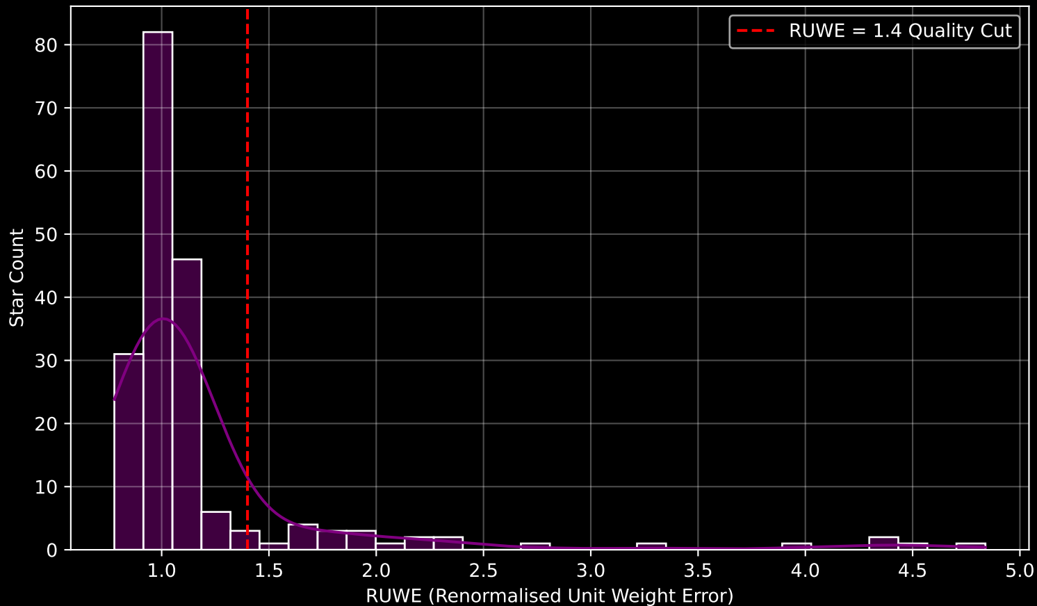
GAPOGEE DR17 Field [077+45_MGA] RUWE Distribution (n= 191)
