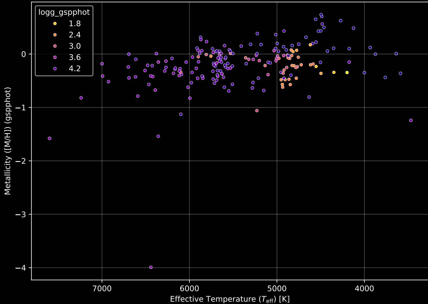
APOGEE DR17 Field: [077+45_MGA] Stellar Population Parameters (n= 196)
