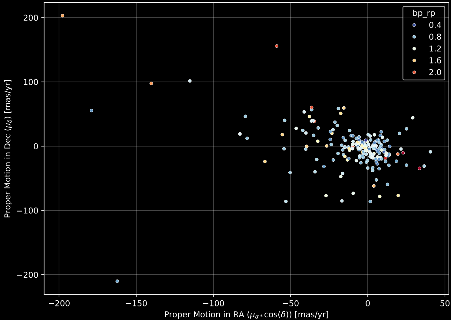
APOGEE DR17 Field: [077+45_MGA] Proper Motion Diagram (n= 196)
